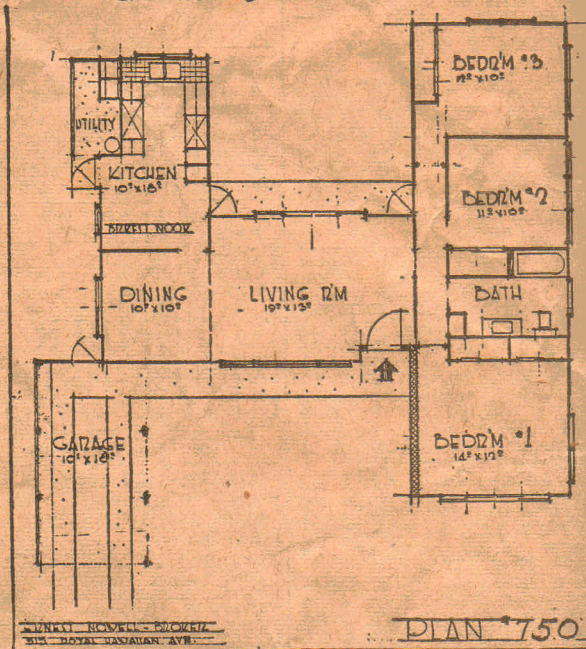
SAMPLE 3 BEDROOM PLANS
