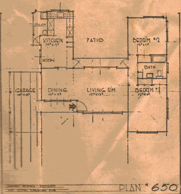
SAMPLE 2 BEDROOM PLANS
